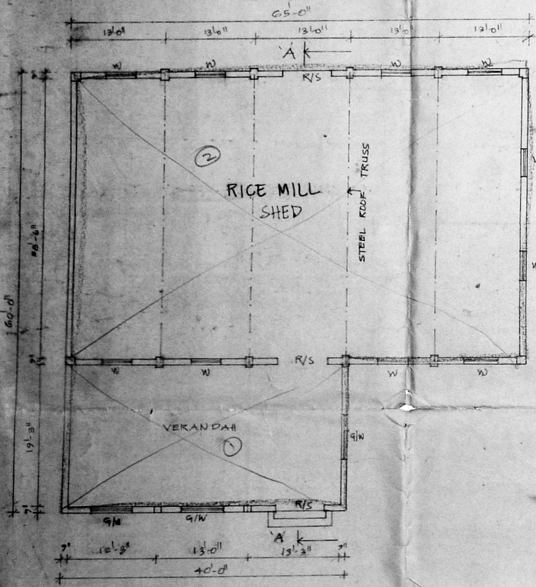
PLAN OF RICE MILL SHED
