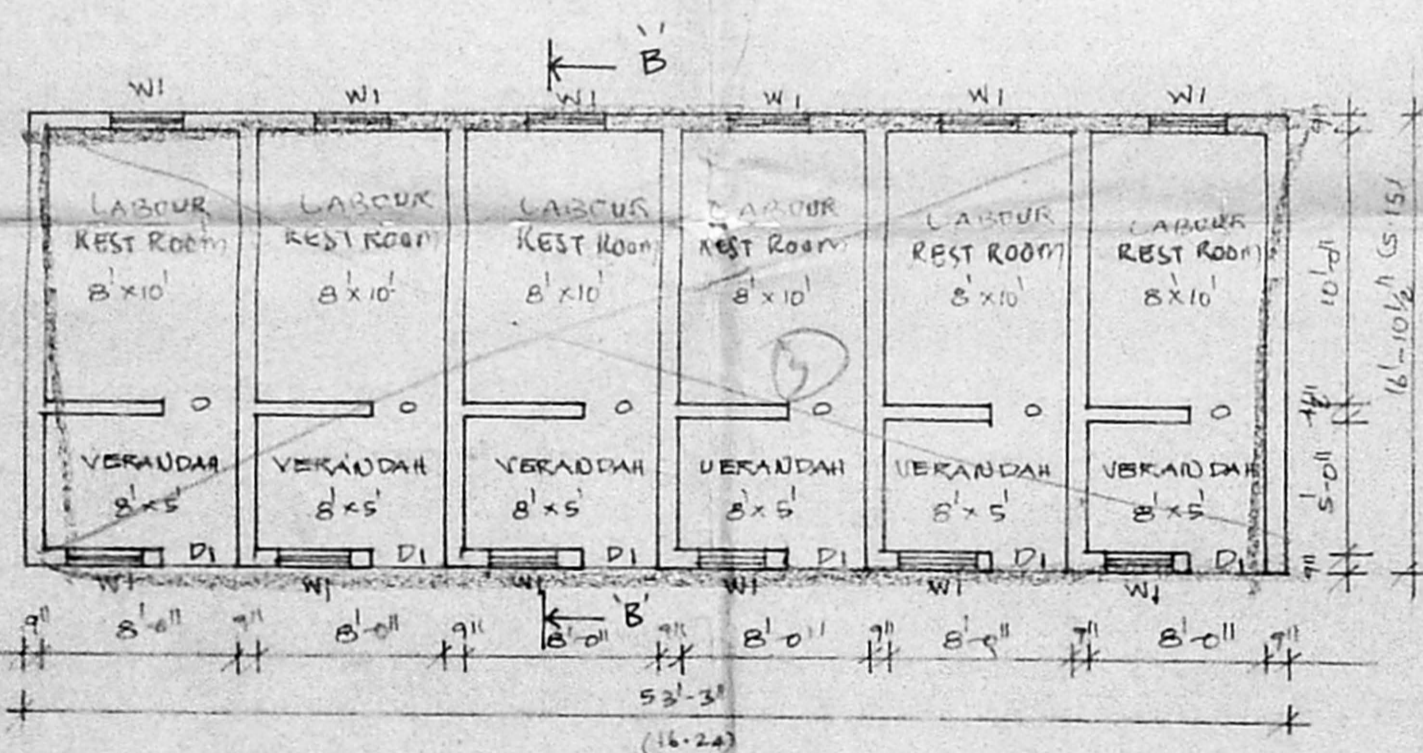
PLAN OF LABOURERS ROOMS (WORKERS ROOMS)
